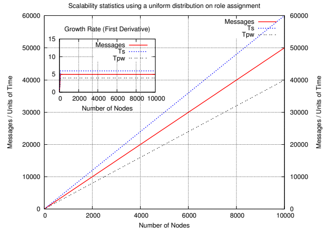
Fig. 6: Statistics with uniform distribution on role assignment
