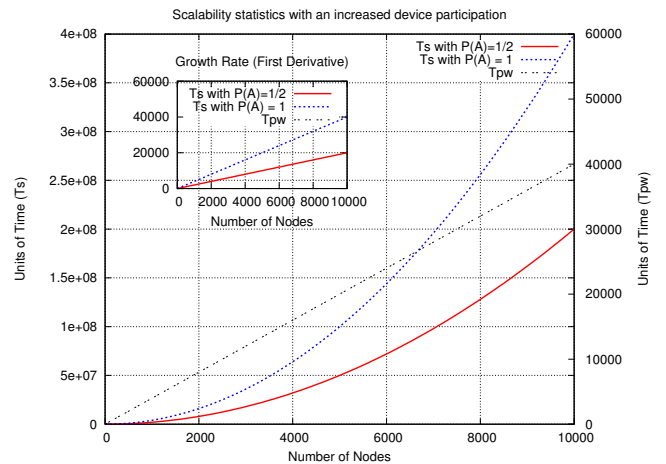
Fig. 7: Statistics with an increased device participation
