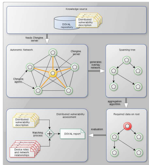
Fig. 4: Overall architecture
